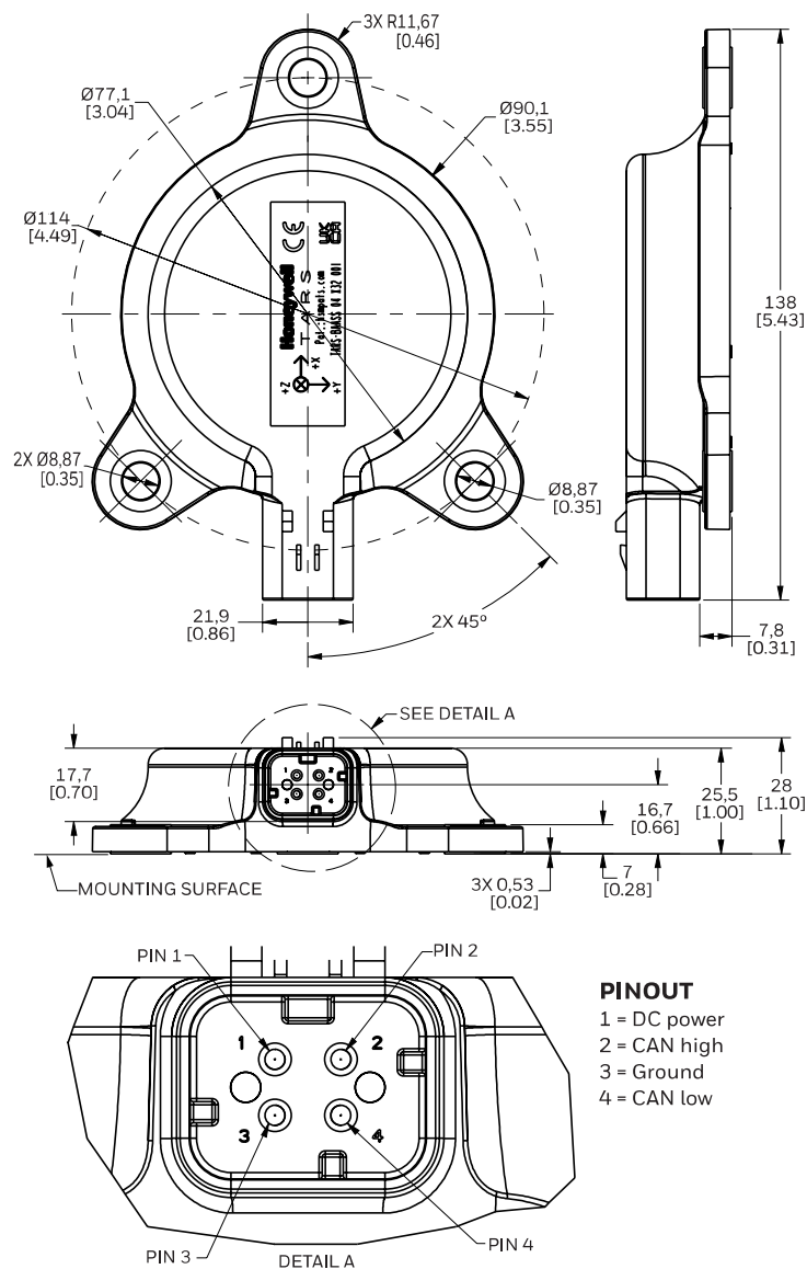
FIGURE 3. BODY DIMENSIONS (FOR REFERENCE ONLY: mm [in])
